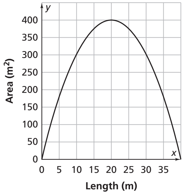
Graph for a Quadratic Relationship
