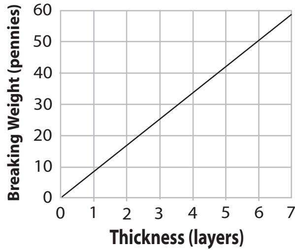
Graph for a Linear Relationship
