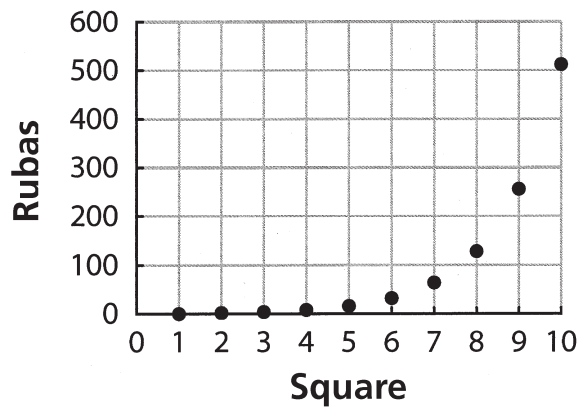
Graph for an Exponential Relationship
